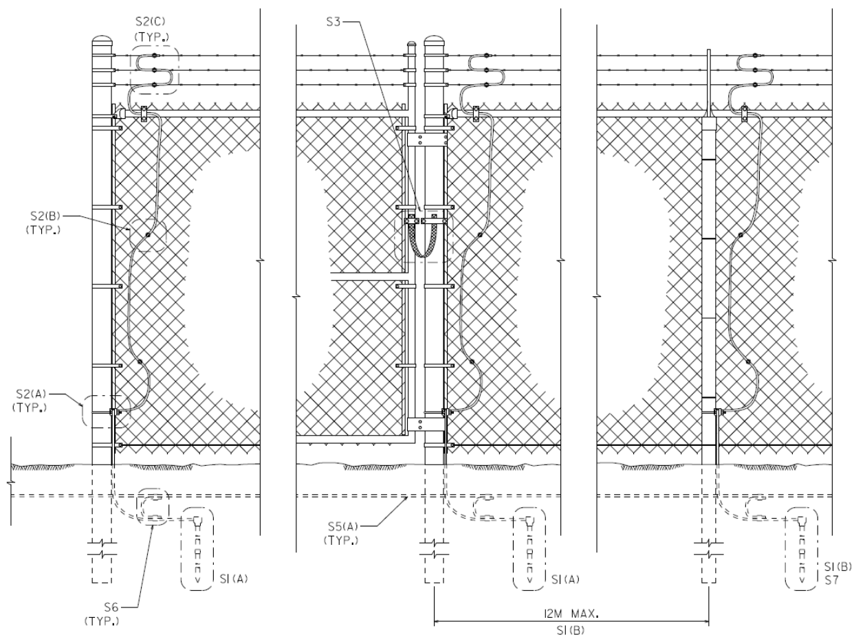
Figure 8 ~ Typical Substation Fence Grounding Application
