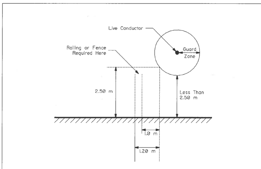
Figure 4 ~ Guarding of Live Parts
