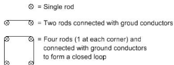
Figure 2 ~ Examples of Ground Electrodes (See Appendix D.)
