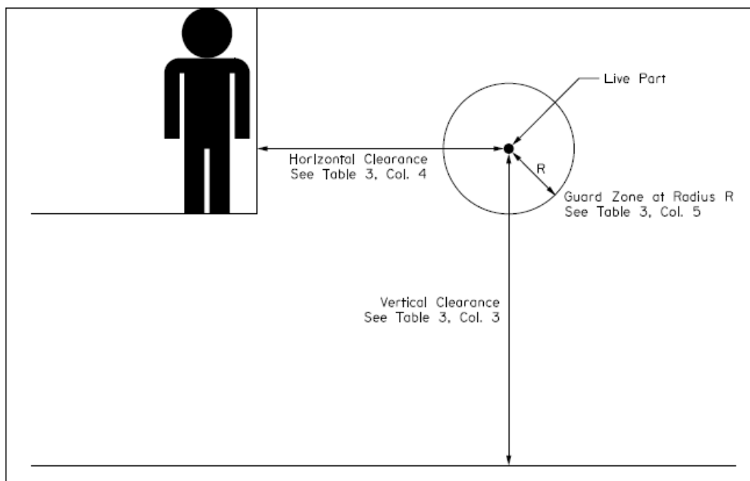
Figure 3 ~ Minimum Clearances about Live Parts (See Table 3.)
