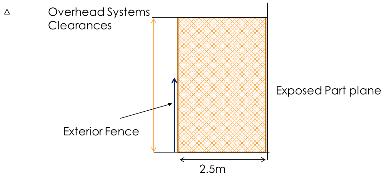
Figure 6 ~ Substation Fence Horizontal Separation for Exposed Parts
