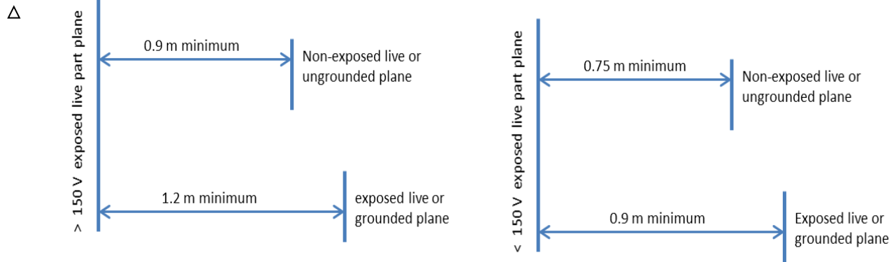
Figure 5 ~ Dimensions of Working Space near Live Parts on Panelboards and Control Panels Indoors
